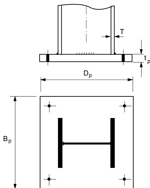
UNIVERSAL COLUMN BASE PLATE DETAILS
