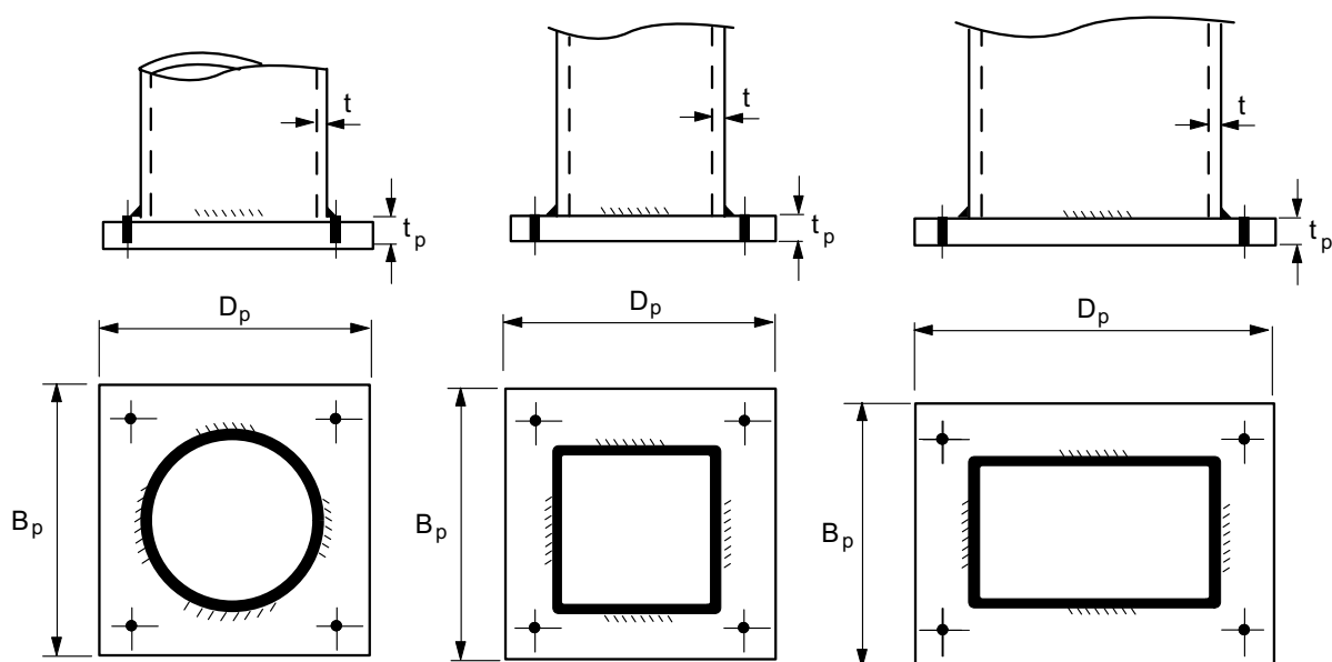
HOLLOW SECTION COLUMN BASE PLATE DETAILS
