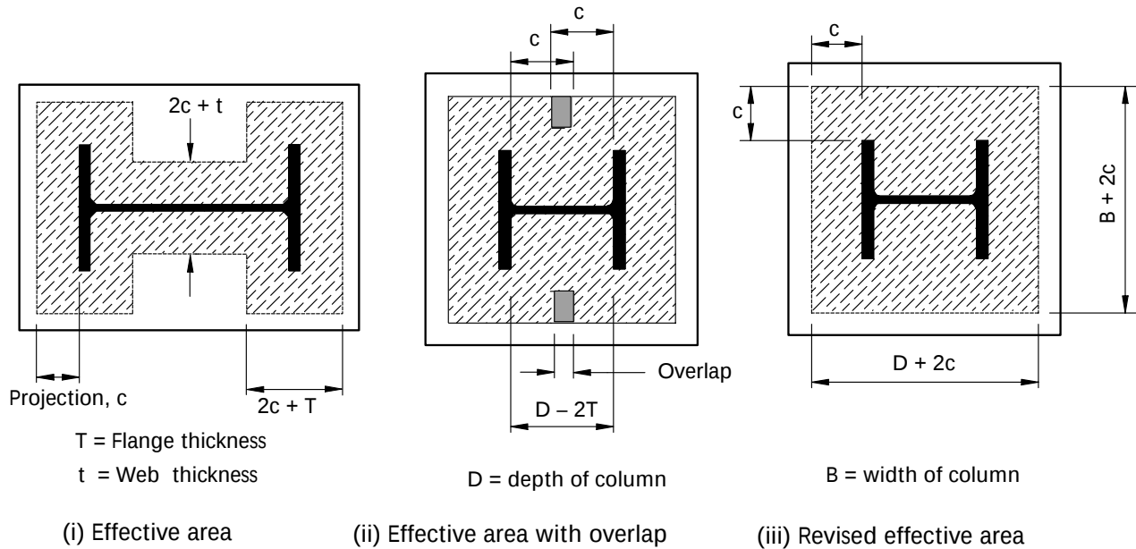
Figure 8.3 Calculated effective area for a rolled section
