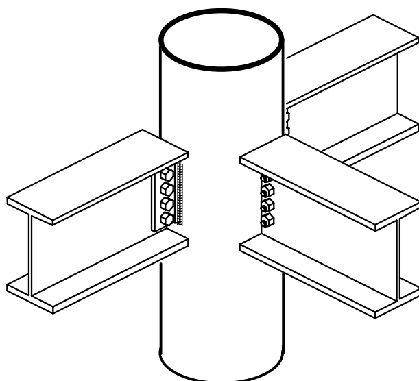
Figure 6.1 Fin plate. Beam-to-column and beam-to-beam connections
