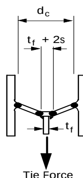
Fin plate connecting to column web
