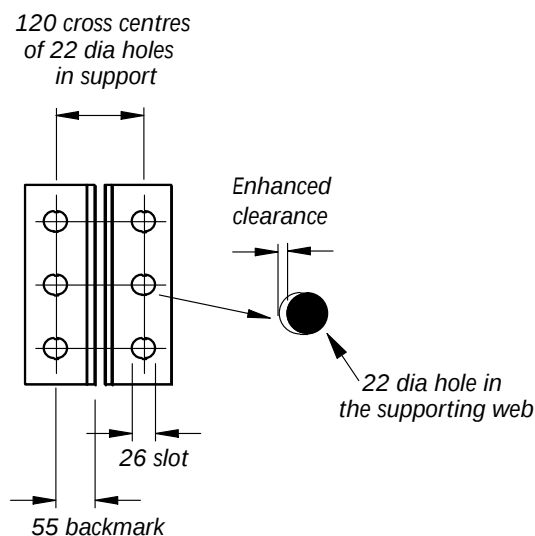
Figure 4.3 Short slotted holes in Double Angle Cleats
