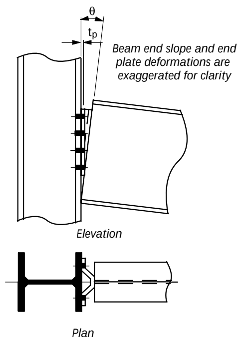
Figure 5.6 Behavior of flexible end plate connections
