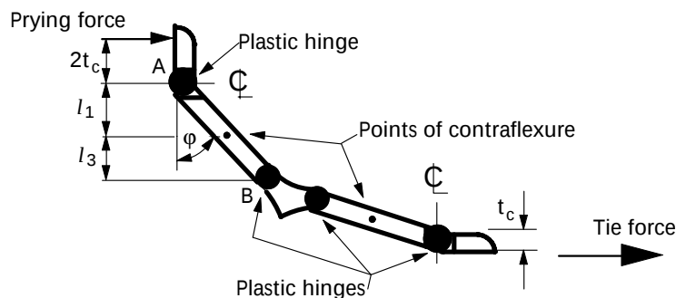
Figure D.1 Web angle cleat under tension
