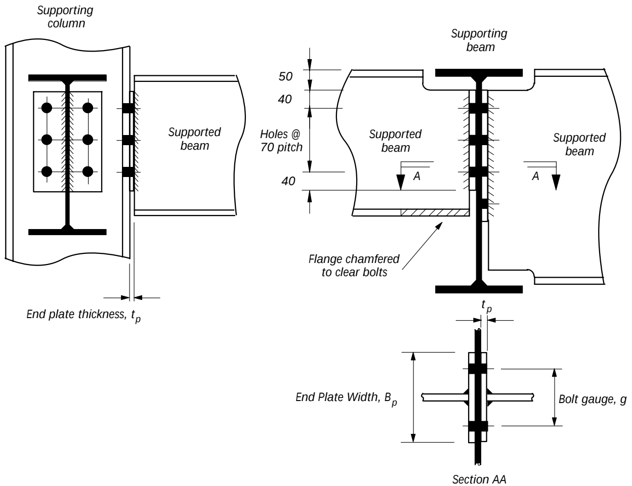
Beam-to-column
