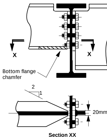
Figure 2.3 Flange chamfers
