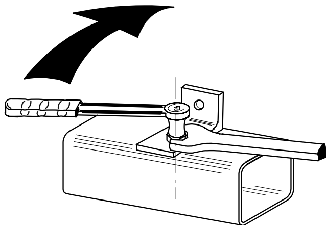
Figure G.5 Installation of Hollo-Bolt
